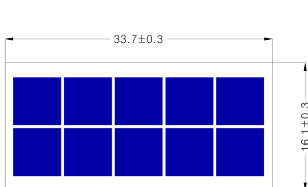
Front-side View
